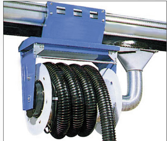
Sliding crabs eliminate the need for overhead drops at every service bay. They are easily positioned wherever needed.
